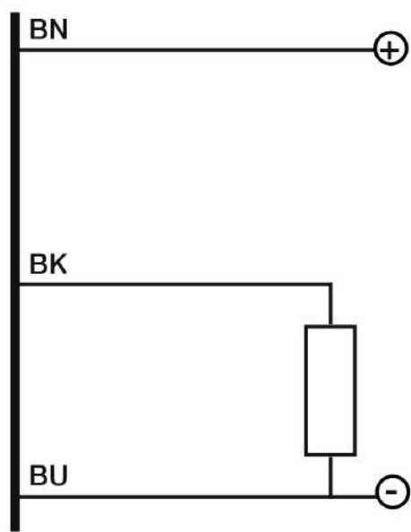
Eletrical diagram
